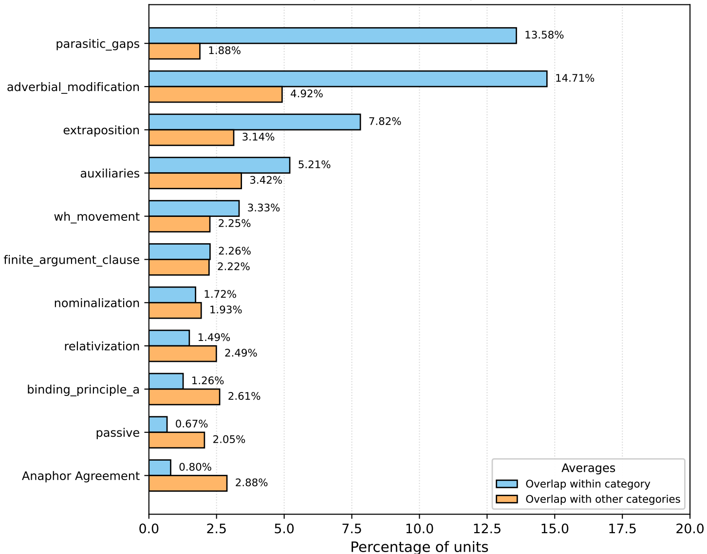
Cross-phenomenon overlap in BLiMP-NL
